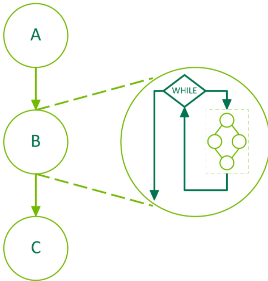
Figure 24: Conditional WHILE Node
