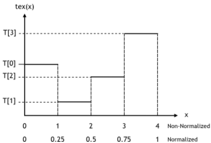
Figure 36: Nearest-Point Sampling Filtering Mode
