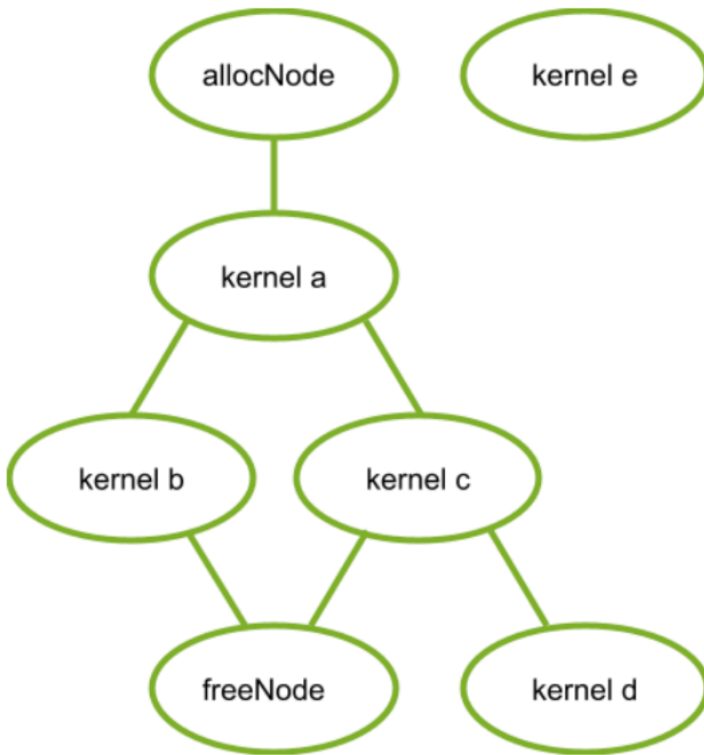
Figure 32: Kernel Nodes
