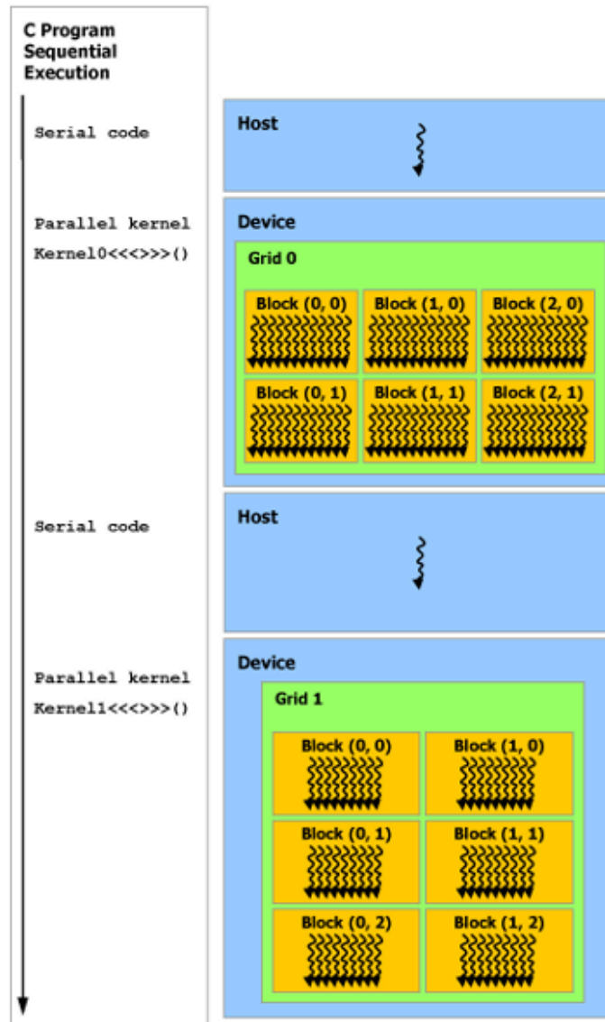
Figure 7: Heterogeneous Programming
