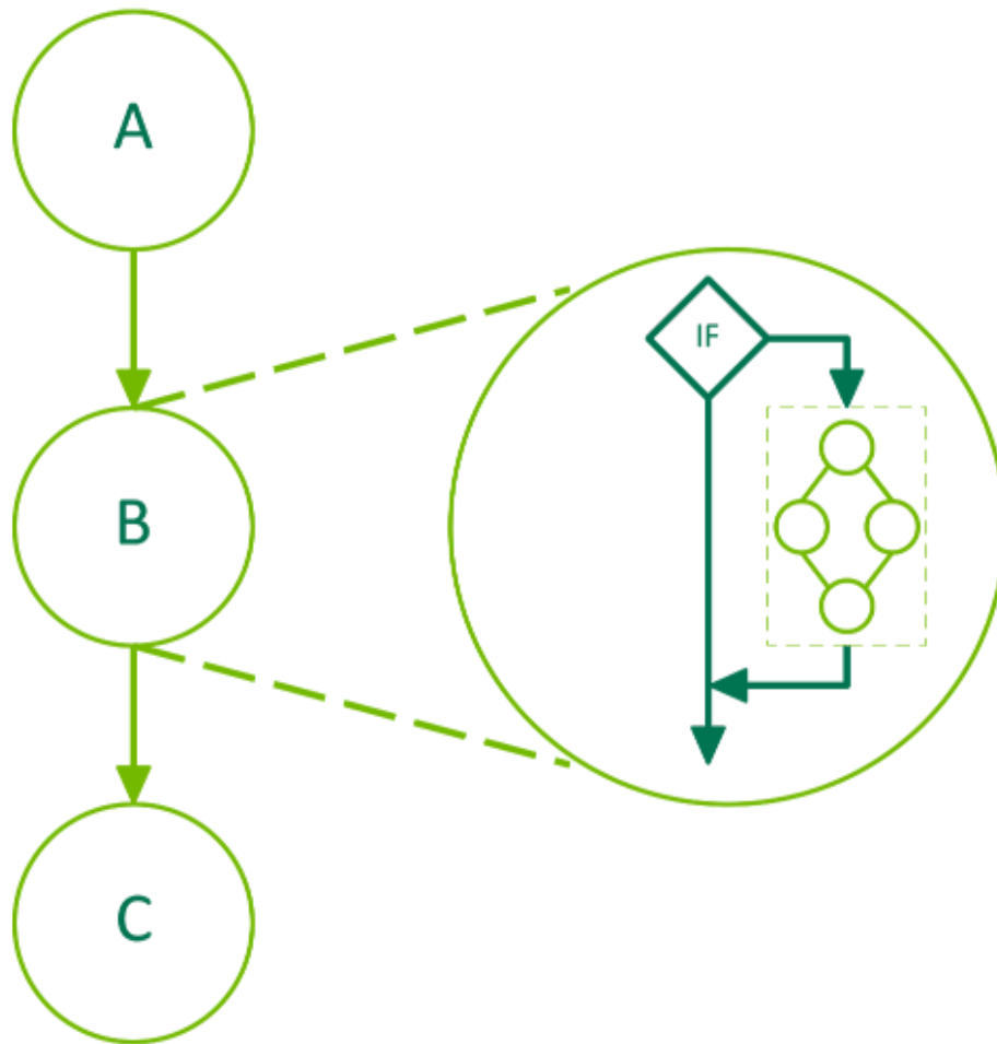
Figure 23: Conditional IF Node
