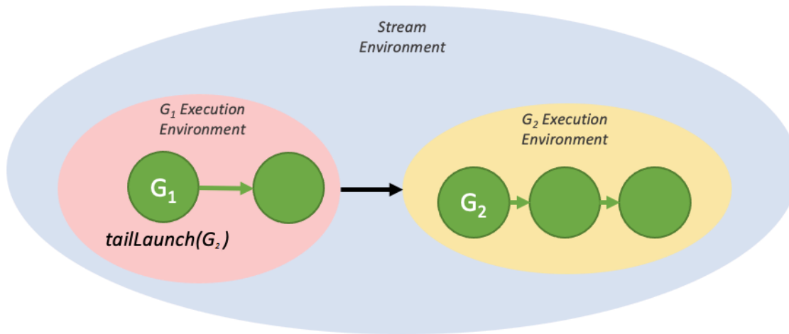
Figure 19: A simple tail launch
