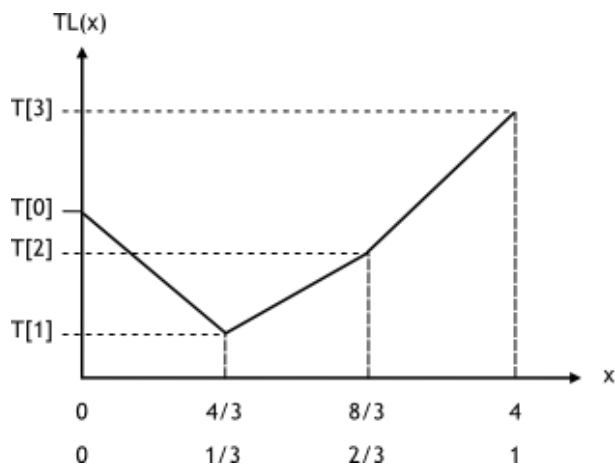
Figure 38: One-Dimensional Table Lookup Using Linear Filtering
