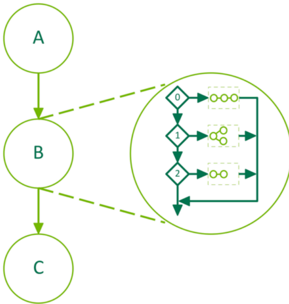
Figure 25: Conditional SWITCH Node
