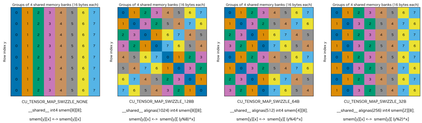
Figure 29: An Overview of TMA Swizzle Patterns
