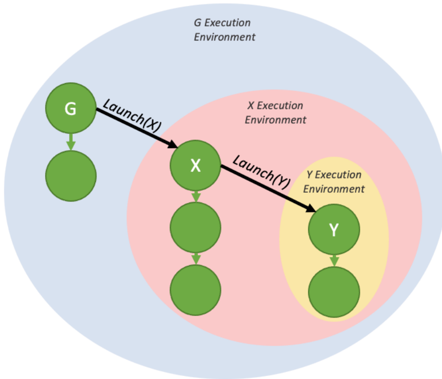
Figure 17: Nested fire and forget environments
