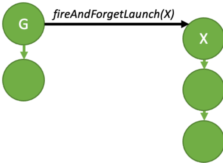
Figure 15: Fire and forget launch
