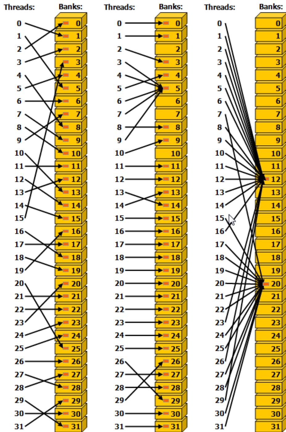
Figure 40: Irregular Shared Memory Accesses.
