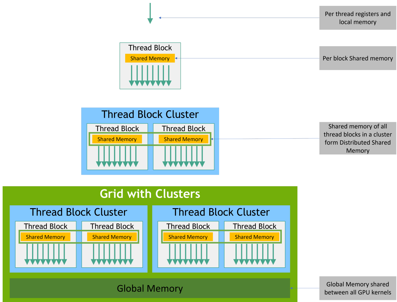
Figure 6: Memory Hierarchy
