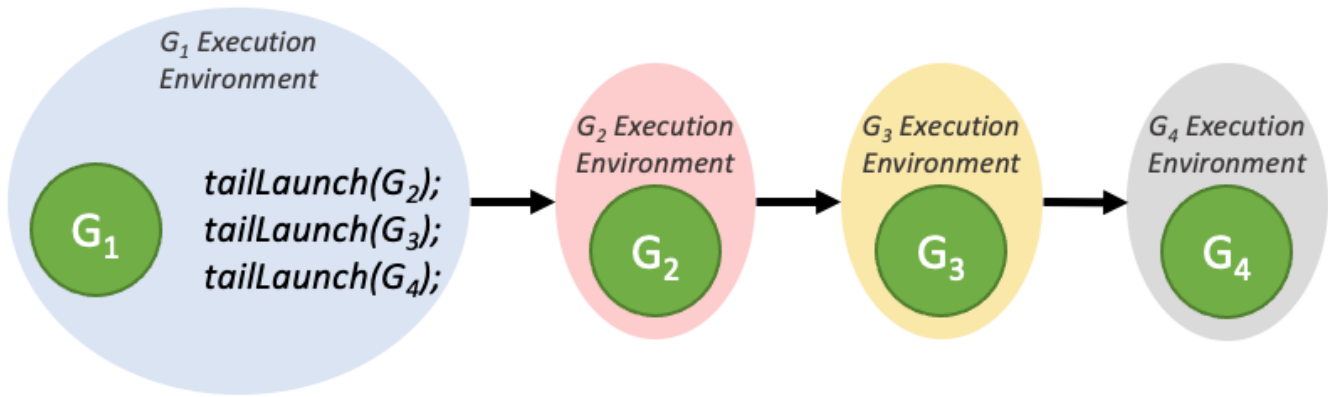
Figure 20: Tail launch ordering
