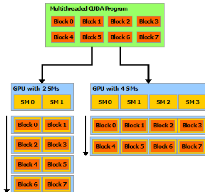
Figure 3: Automatic Scalability
