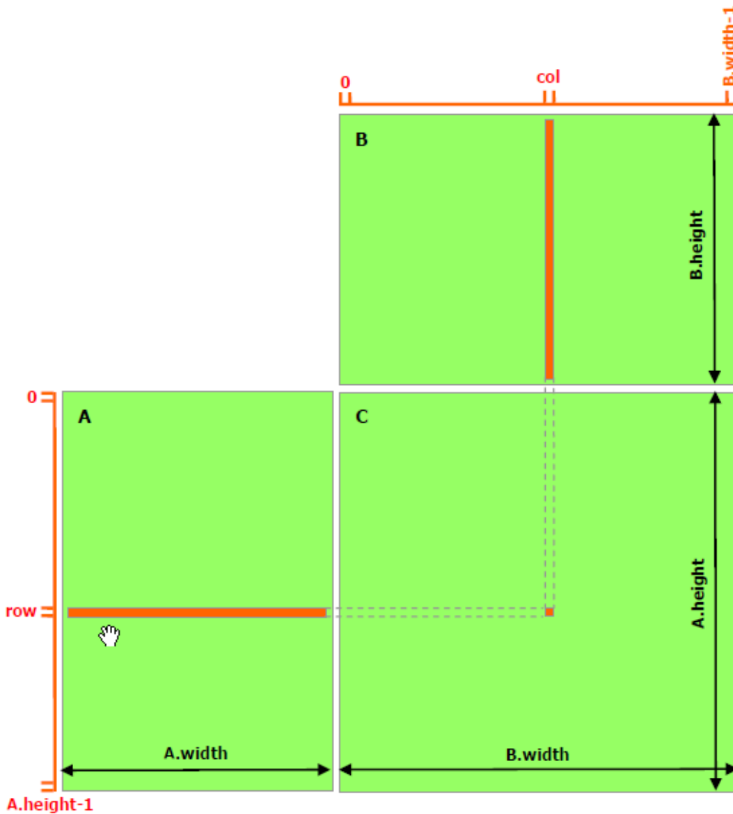
Figure 8: Matrix Multiplication without Shared Memory
