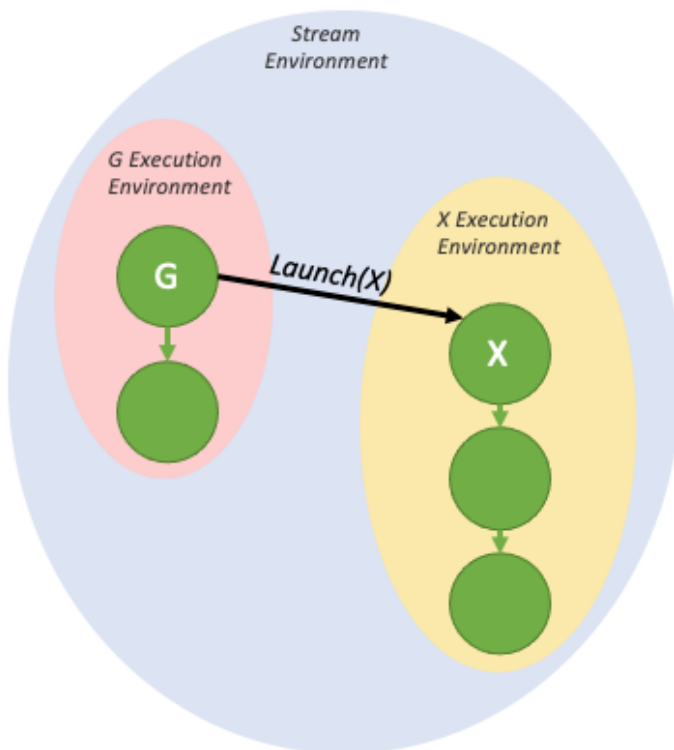
Figure 22: A simple sibling launch
