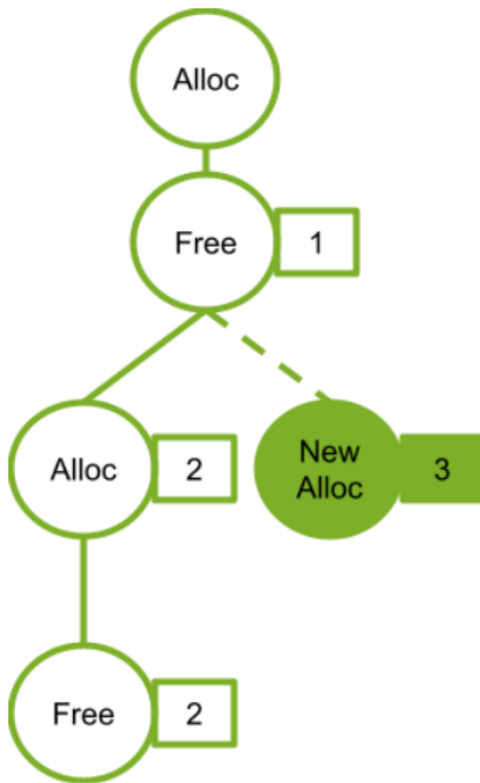
Figure 34: Adding New Alloc Node 3
